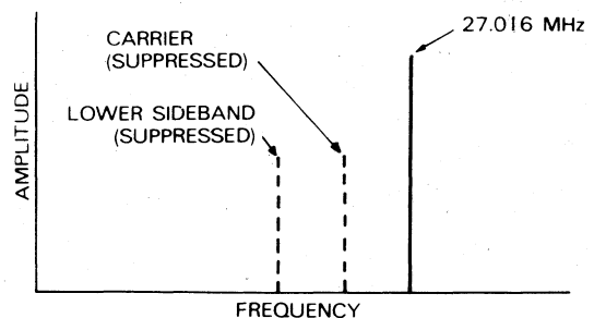
SSB UPPER SIDEBAND
