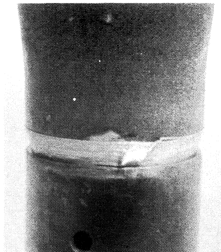
Fig.1B: Wrap a layer of 5A fusewire around the damaged shielding and solder to the earthing wire.
