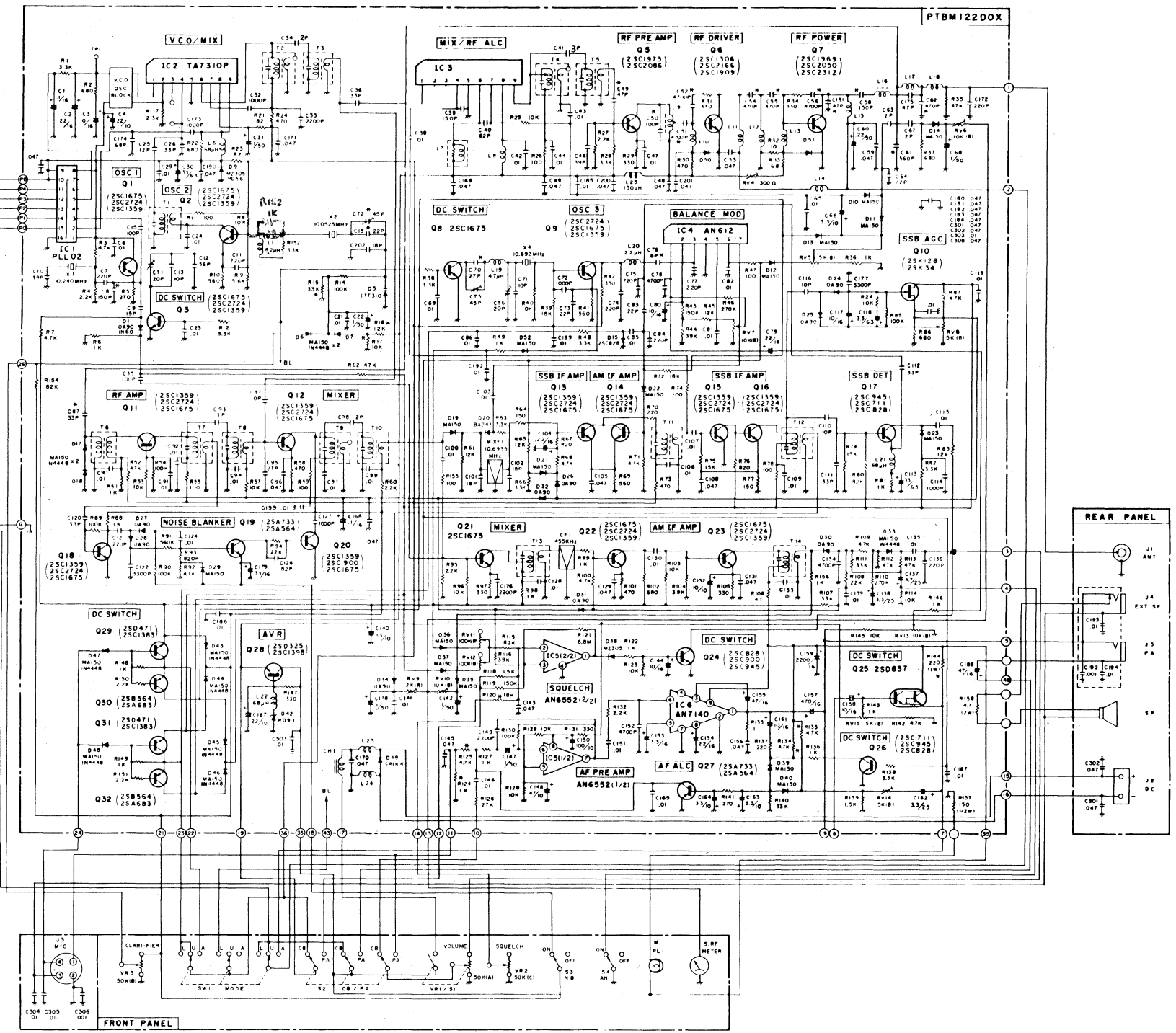
Schematic Diagram
