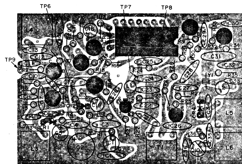
DIGITAL SYNTHESIZER BOARD (SOLDER SIDE VIEW) 37-0194-022
