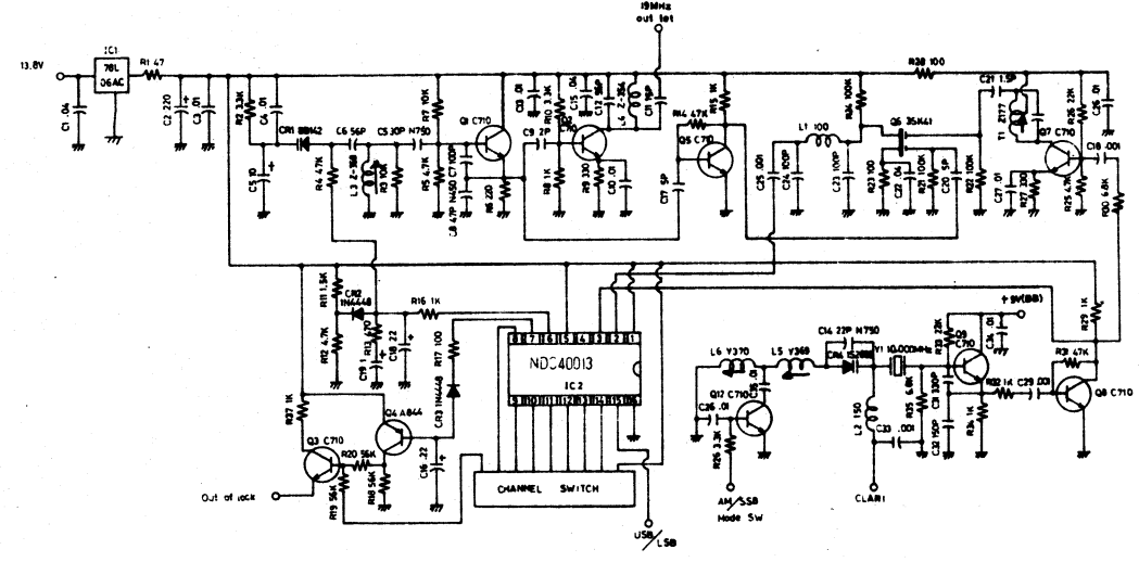
DIGITAL SYNTHESIZER SCHEMATIC DIAGRAM
