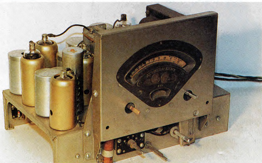
Fig.7: The 1934 model 447 chassis has some features found more often in a communication receiver, including continuous coverage from 550kHz to 23MHz in four bands. The RF stage is used on all bands and each band has an oscillator padder, ensuring accurate dial readings and tracking.
