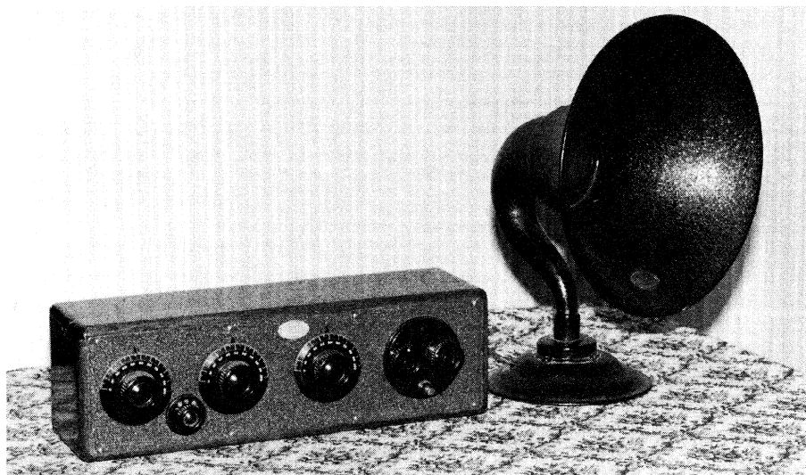
Fig.1: The attractive little 1926 model 20C was a hit with the ladies, and is the oldest A-K model commonly found in Australasia. Whereas contemporary loudspeakers commonly had aluminium or paper-mache flares, Atwater Kent made his of heavy gauge steel!
